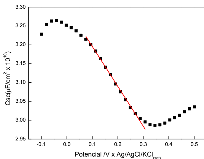
Fig. 2. MSP curve for the heavily BDD/Ti sample.
